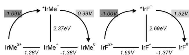
Scheme 2. Latimer diagrams for the IrMe and IrF complexes based on the electrochemical and spectroscopic data from Table 2.
