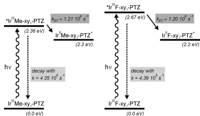
Scheme 3. Schematic diagrams illustrating the energetics and kinetics of the photoinduced processes occurring in the IrMe-xy 1 -PTZ and IrF-xy 1 -PTZ dyads.
