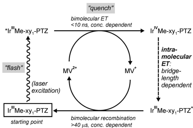
Scheme 4. Illustration of the flash-quench technique used to induce phenothiazine-to-Ir IV electron transfer in the IrMe-xy 1 -PTZ dyad.
