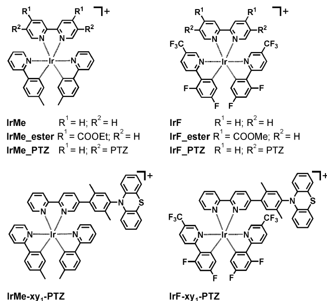
Scheme 1. Formulas of the molecules investigated in this work.
