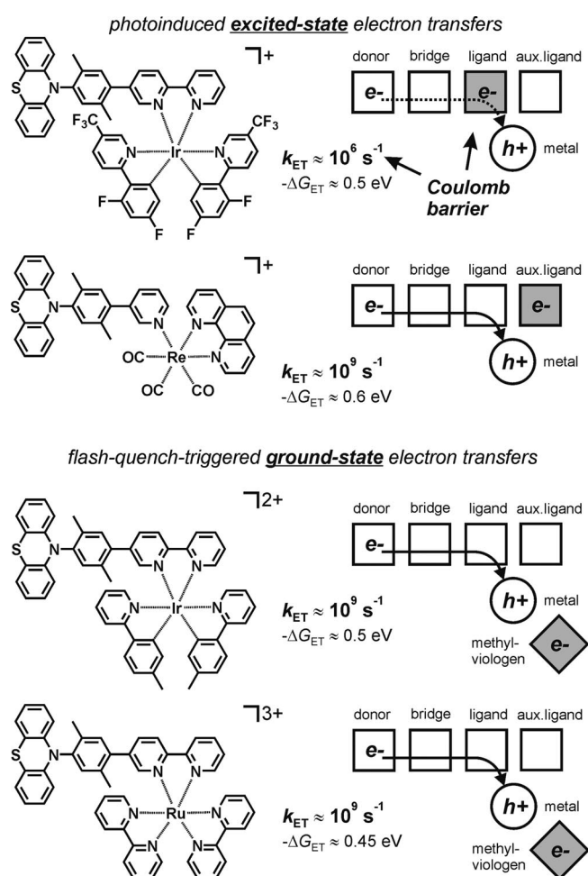
Scheme 5. Excited-state PTZ-to-Ir III electron transfer is slow in the IrF-xy 1 -PTZ and IrMe-xy 1 -PTZ dyads (top). In an analogous rhenium(I)-based dyad (second from top), the PTZ-to-Re I excited-state electron transfer is three orders of magnitude faster despite identical donor–acceptor distance and similar driving force ( -\Delta G_{ET} ), but in this case the MLCT excitation does not impose a Coulomb barrier to long-range electron transfer. Ground-state PTZ-to-Ir IV and PTZ-to-Ru III electron transfers across the same distance and similar -\Delta G_{ET} are also three orders of magnitude faster (bottom half), because in this case the MLCT excited electron is abstracted by methylviologen and there is no Coulomb barrier associated with long-range electron transfer either.
