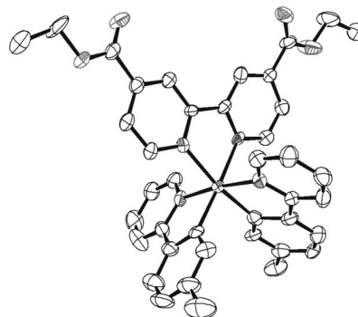
Figure 1. Crystal structure of the IrMe_ester complex. The thermal ellipsoids for the image represent the 50% probability limit. All hydrogen atoms are omitted for clarity.
