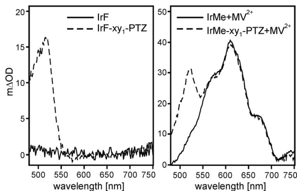
Figure 3. Left: transient absorption spectra obtained from 0.1 mM solutions of IrF and IrF-xy 1 -PTZ following excitation at 457.9 nm with 10-ns laser pulses. [24] Detection occurred in a time window ranging from 2 to 12 μs after the laser pulse. Right: transient absorption spectra measured on deoxygenated acetonitrile solutions containing 0.1 mM iridium complex (IrMe or IrMe-xy 1 -PTZ) and 50 mM methylviologen (MV 2+ ). Excitation occurred at 457.9 nm with laser pulses of ca. 10 ns duration, detection occurred in a 10-μs time window starting 500 ns after the excitation pulse.
