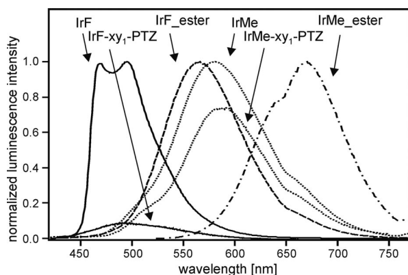
Figure 2. Luminescence spectra obtained from room-temperature acetonitrile solutions of the six emissive complexes from Scheme 1. Excitation occurred at 390 nm. Emission intensities are normalized, and only the IrF/IrF-xy 1 -PTZ and the IrMe/IrMe-xy 1 -PTZ intensities can be compared mutually.
